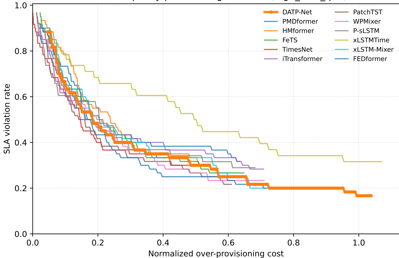
GÉANT capacity provisioning trade-off (high_load_q90)
