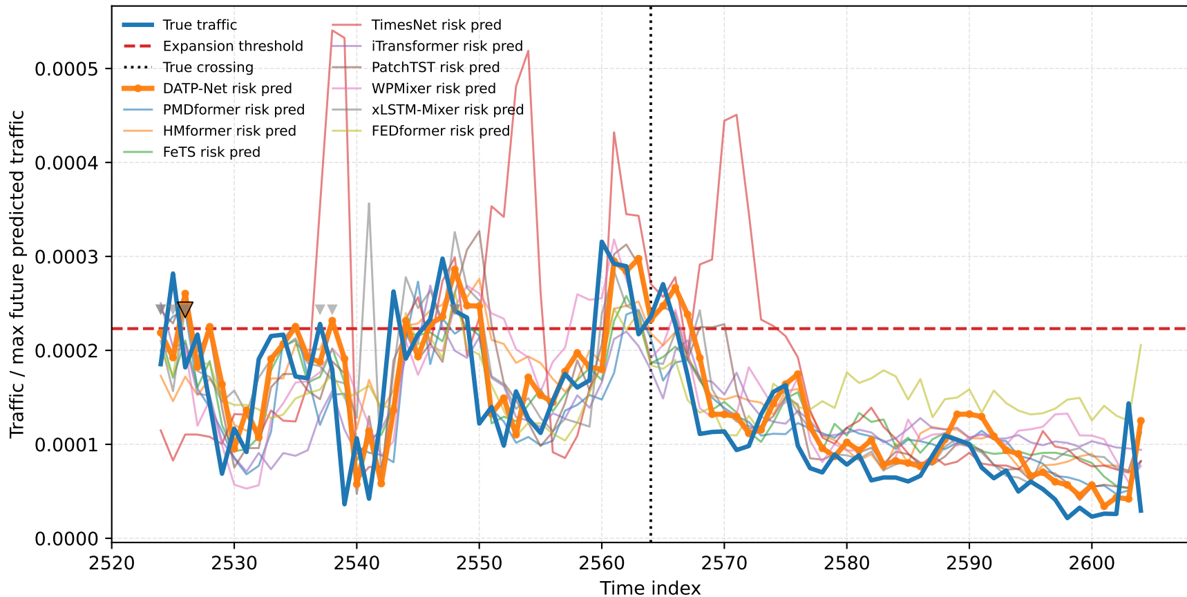
Abilene turning-point early warning case 1
