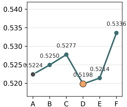
State Prior Scales
