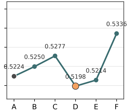
State Prior Scales
