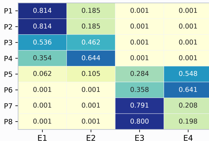
Abilene Sample 2 (id=2320)
