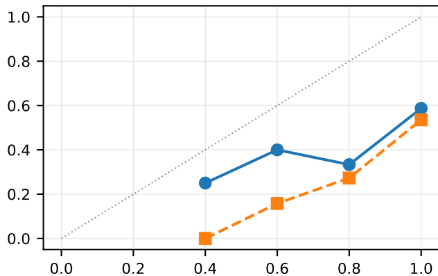
Phi-3.5-mini / TruthfulQA
