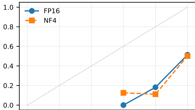
Qwen2.5-3B / TruthfulQA
