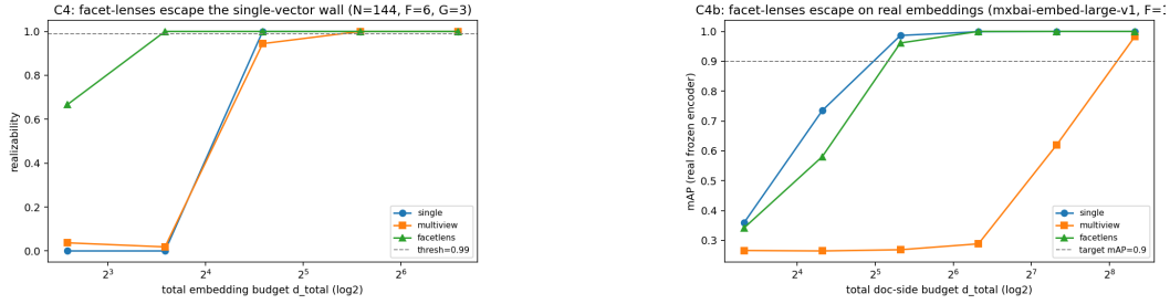
Figure 5: C4 and its scope. Left (free vectors): routed facet-lenses escape the wall at half the budget of a single vector, while generic multiview is worse than single. Right (frozen real encoder): the escape vanishes—a single learned projection ties the routed lenses and leads at tight budgets—because a strong encoder has already linearized the facets.
