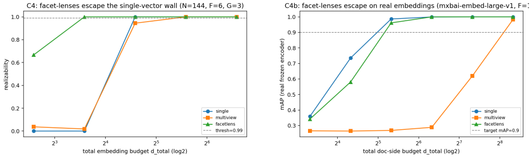
Figure 5: C4 and its scope . Left (free vectors): routed facet-lenses escape the wall at half the budget of a single vector, while generic multiview is worse than single. Right (frozen real encoder): the escape vanishes—a single learned projection ties the routed lenses and leads at tight budgets—because a strong encoder has already linearized the facets.
