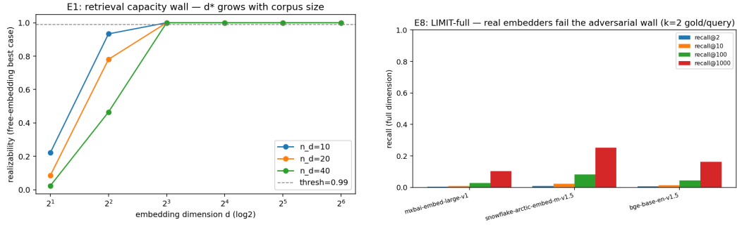
Figure 2: C1 . Left: the free-embedding retrieval wall—realizability jumps sharply once d_r clears a critical value that grows with corpus size n_d . Right: on LIMIT, three real embedder families all fail the adversarial pattern at full dimension.
