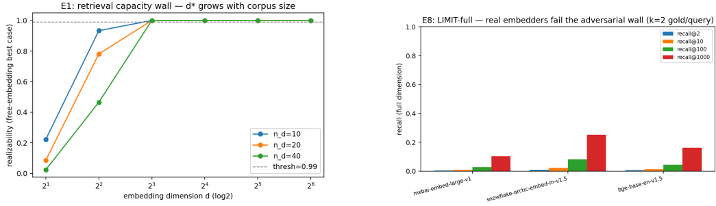
Figure 2: C1 . Left: the free-embedding retrieval wall—realizability jumps sharply once d_r clears a critical value that grows with corpus size n_d . Right: on LIMIT, three real embedder families all fail the adversarial pattern at full dimension.
