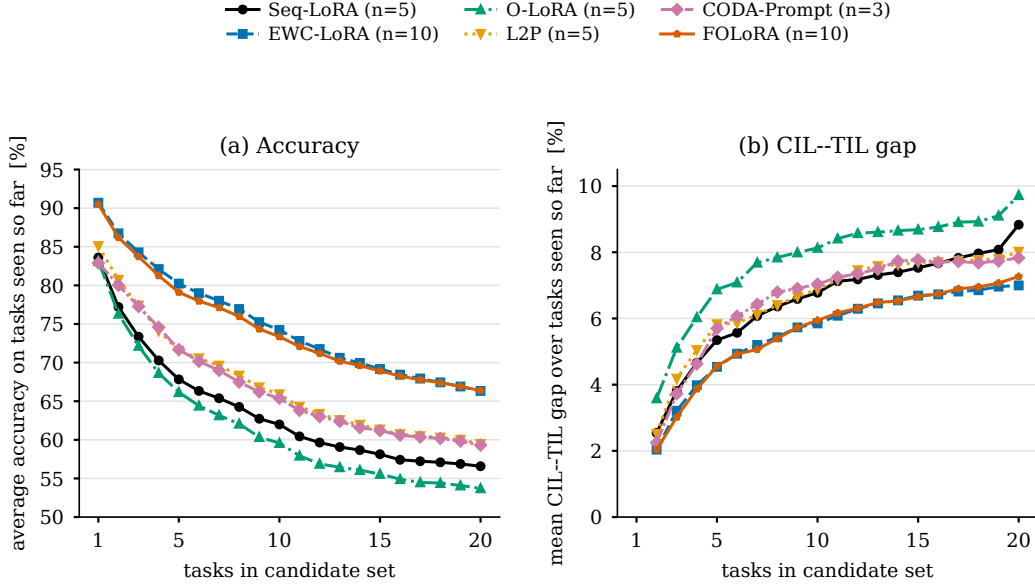
Figure 3: Average accuracy over the candidate classes seen so far (left) and the mean CIL--TIL gap over those candidate sets (right) on Split ImageNet-R. As in Fig. 2, each point is a single feature extraction of the terminal model re-scored against a growing candidate set (10 classes per task, 10 to 200), not a training trajectory. Each curve is drawn at the configuration and the seed budget of its row in Table 1 — CODA-Prompt on three seeds, L2P, O-LoRA and Seq-LoRA on five, EWC-LoRA and FOLoRA on ten — so its right-hand endpoint reproduces that row’s \overline{\text{ACC}} . Those budgets differ between methods (Sec. 5.1), so the legend carries each curve’s n and the figure implies no equal n . No reproducibility-floor band is drawn, because that floor was measured on CIFAR-100 only and we do not transfer it to another dataset. The vertical axis is bounded below at 50, i.e. 3.72 points under the lowest value plotted.
