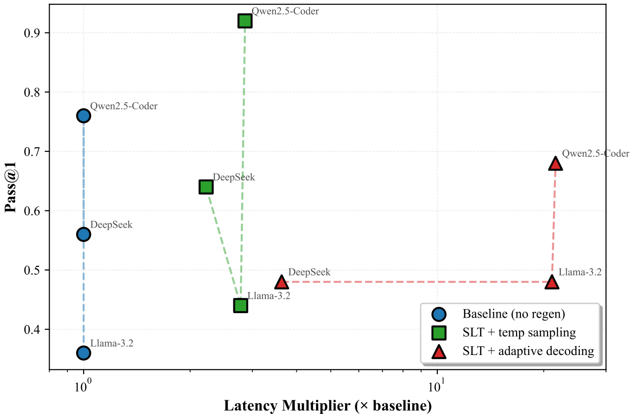
Pass@1 vs Latency Trade-off
