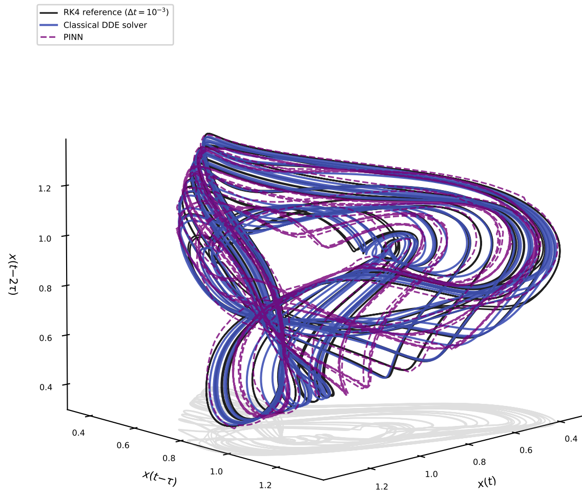
Mackey-Glass ( n = 10 ) (a)
