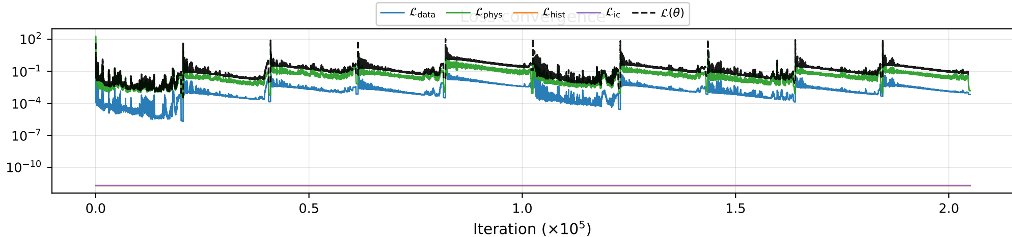
MSE loss terms
