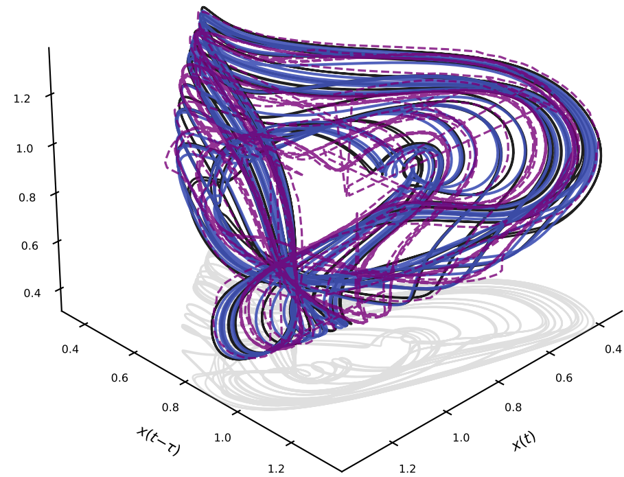
Mackey-Glass ( n = 10 ) (c)
