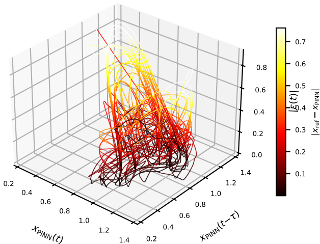
PINN error in delay space ( n = 10 )
