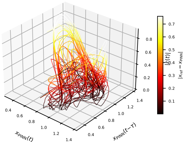
PINN error in delay space ( n = 10 )
