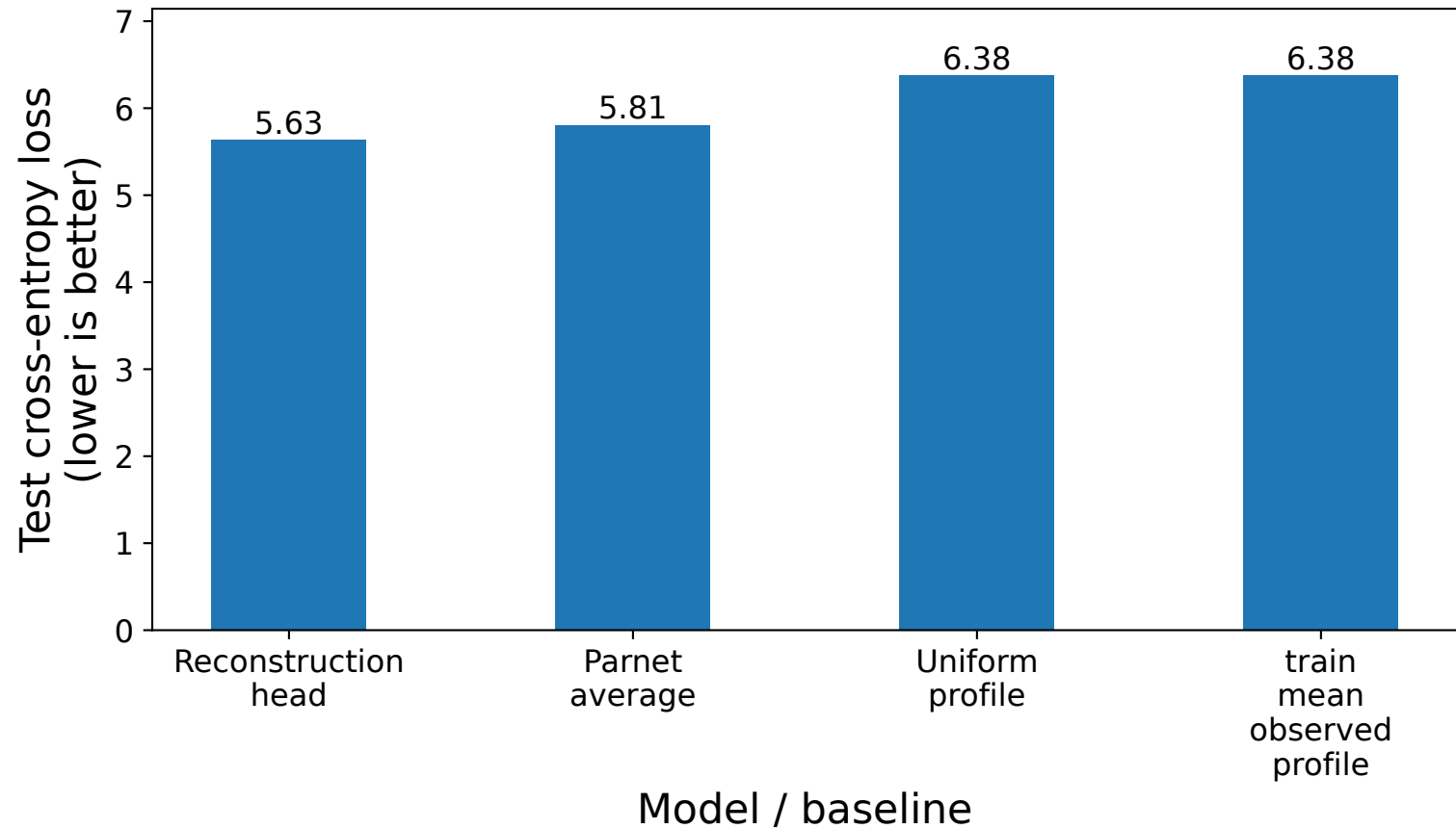
Idea 1 test loss comparison
