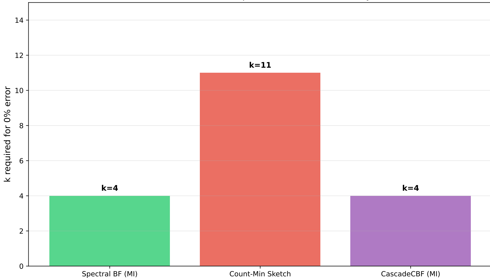
Hash Functions Required for Perfect Accuracy
