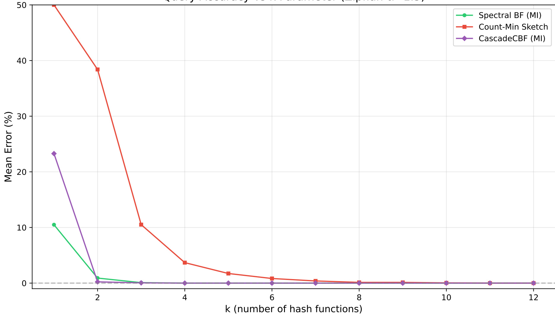
Query Accuracy vs k Parameter (Zipfian \alpha=1.5 )
