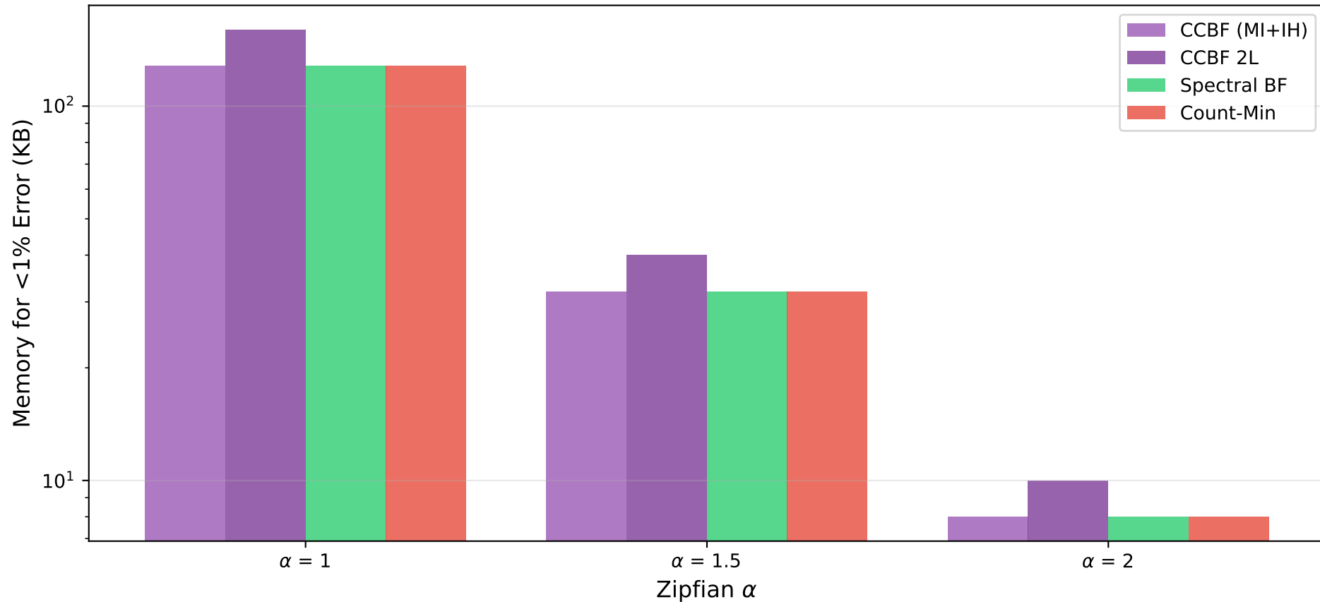
Memory Required to Achieve <1% Mean Error
