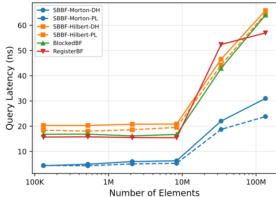
3D Query Performance vs Scale
