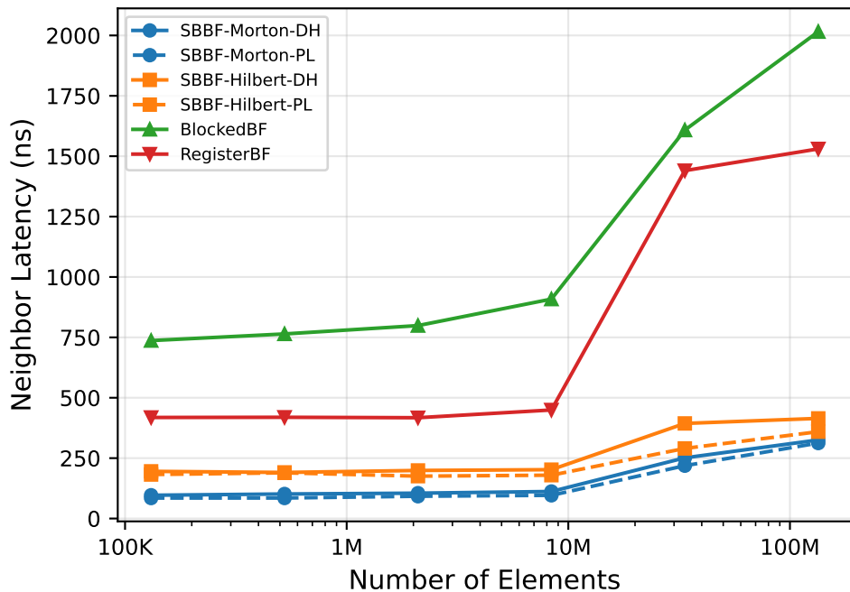
3D Query Performance vs Scale
