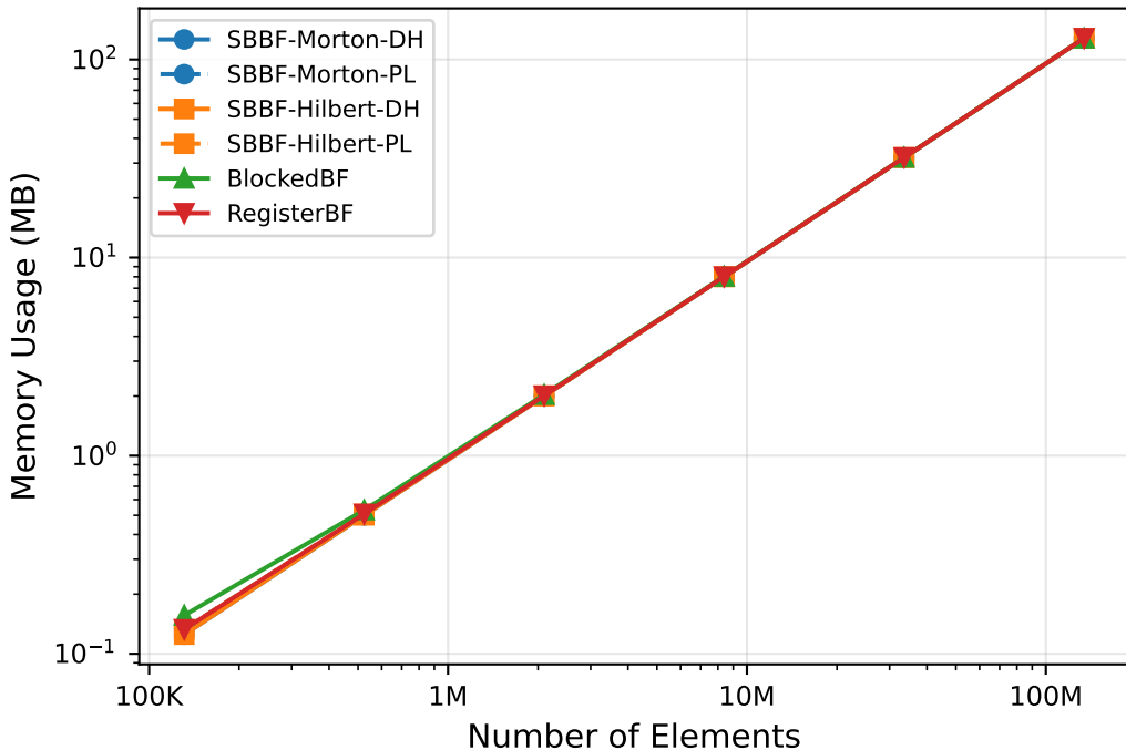
2D Filter Memory Usage vs Scale
