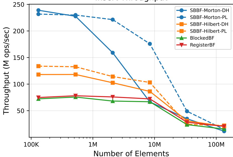
Insert Throughput
