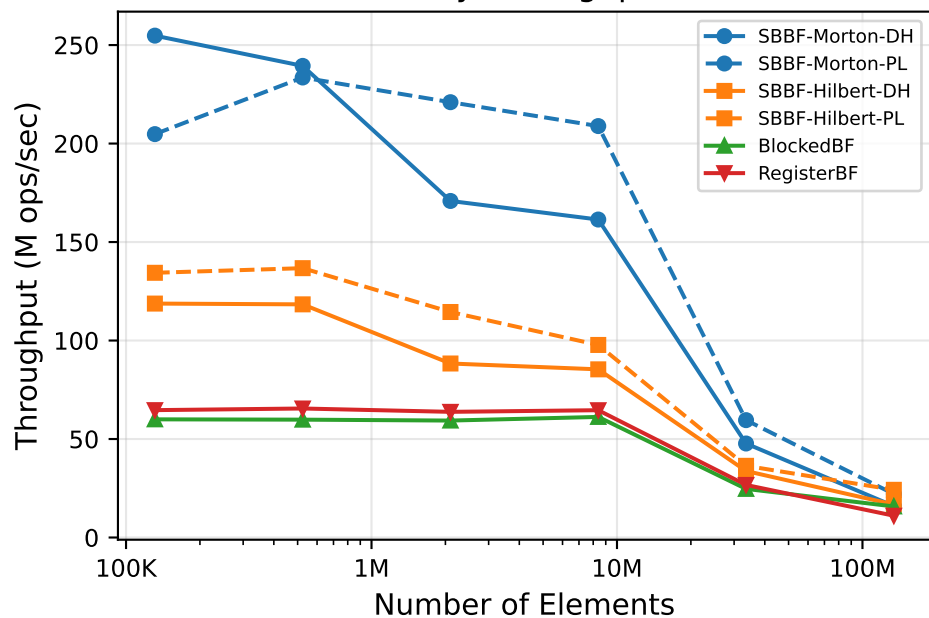
Query Throughput
