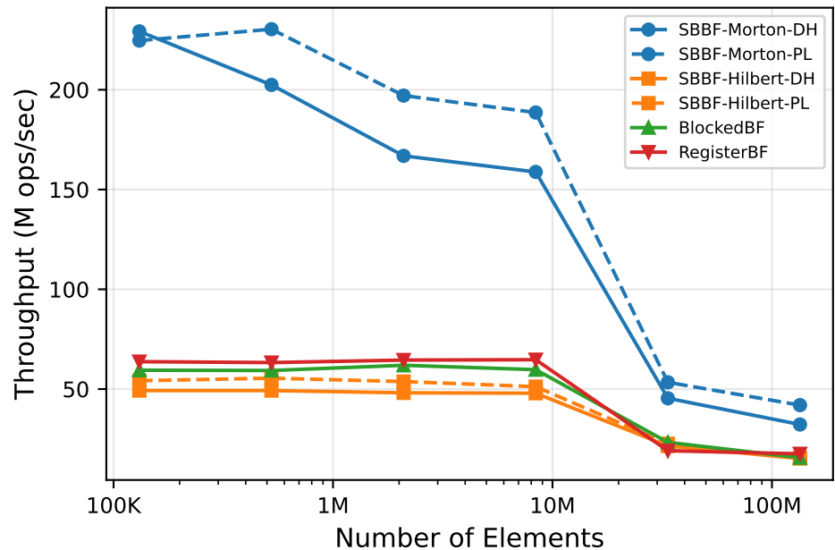
Query Throughput
