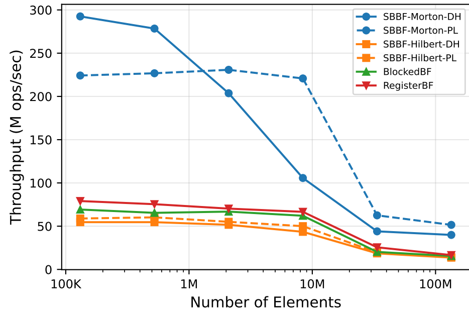
Insert Throughput
