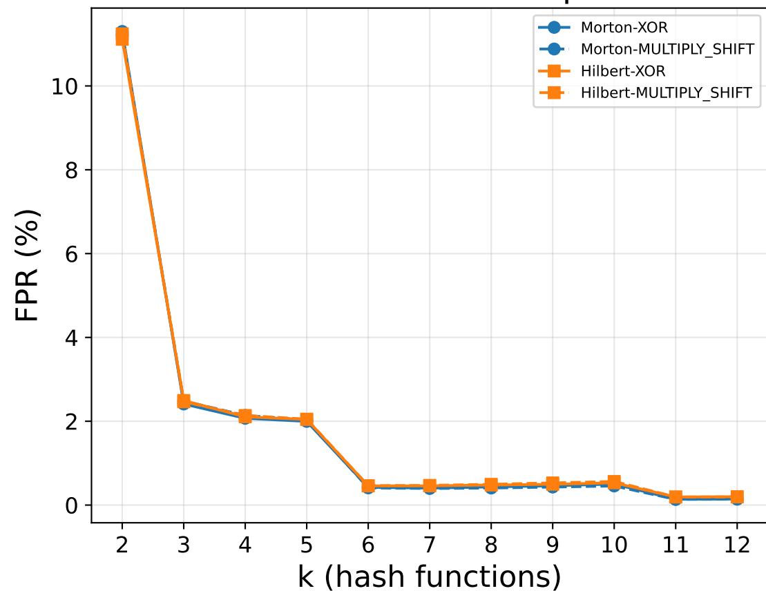
2D Pattern-Lookup
