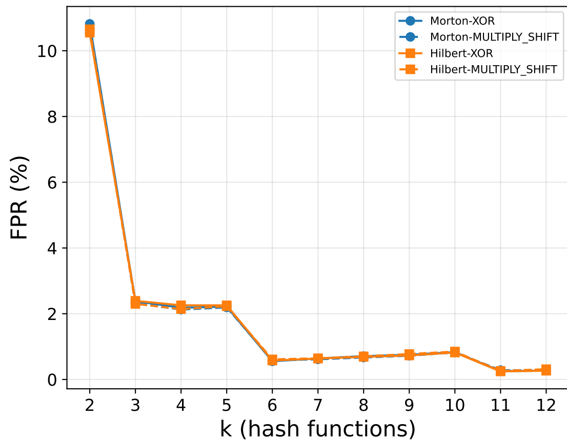
3D Double-Hash
