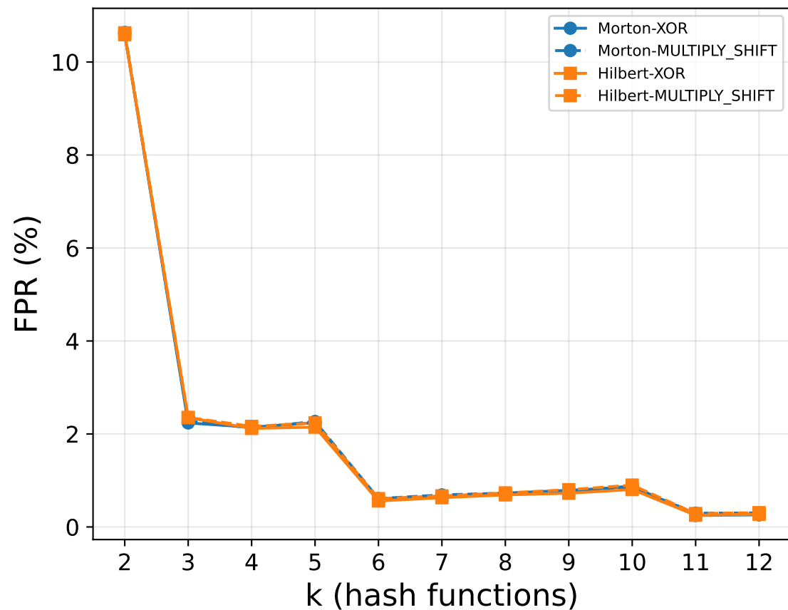
2D Double-Hash
