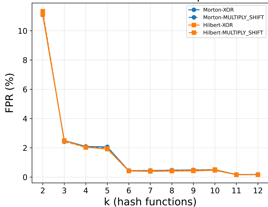
3D Pattern-Lookup
