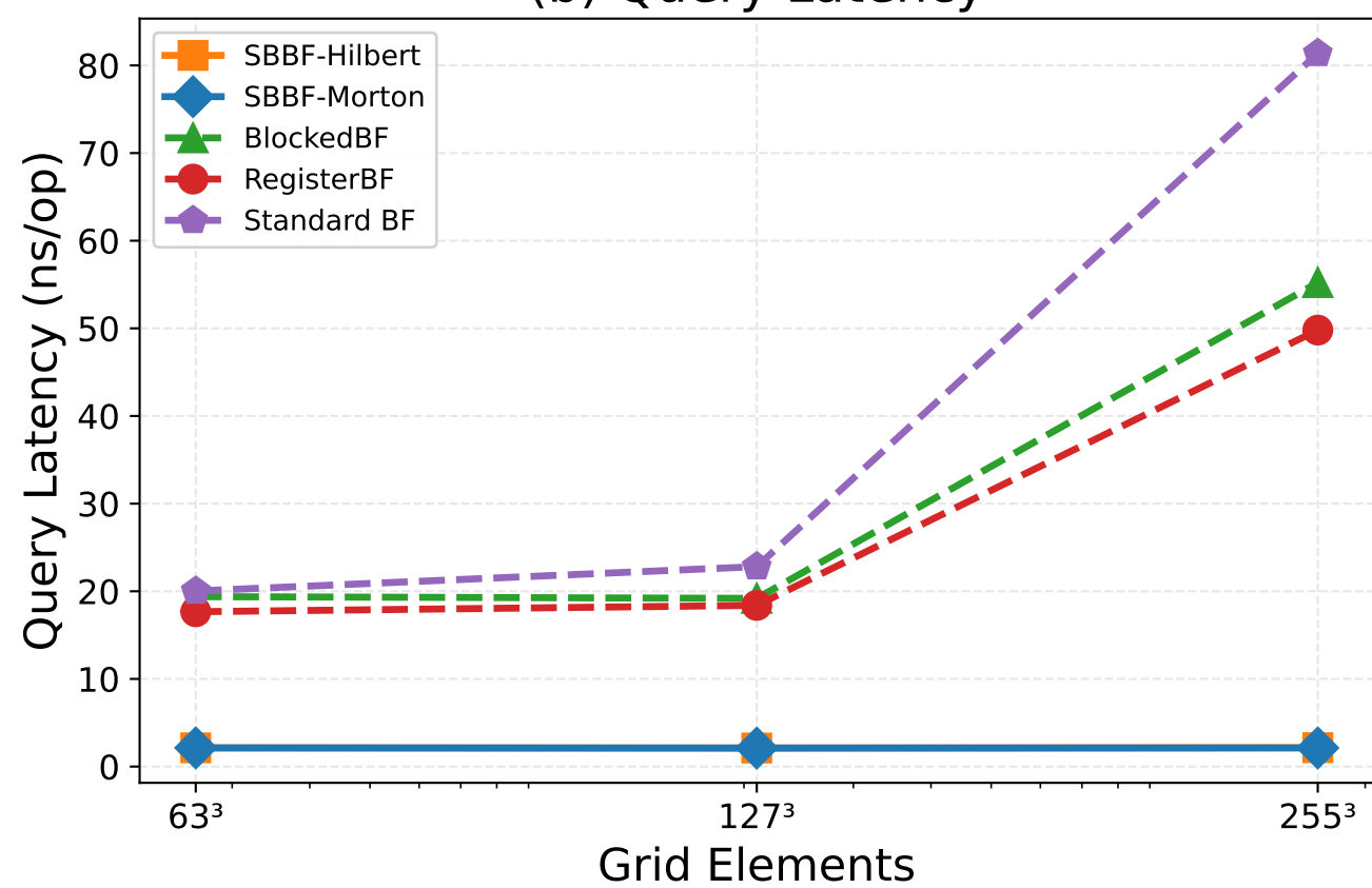
(b) Query Latency
