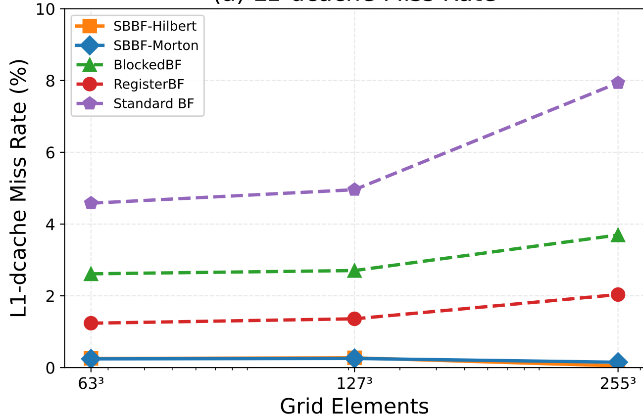
(a) L1-dcache Miss Rate
