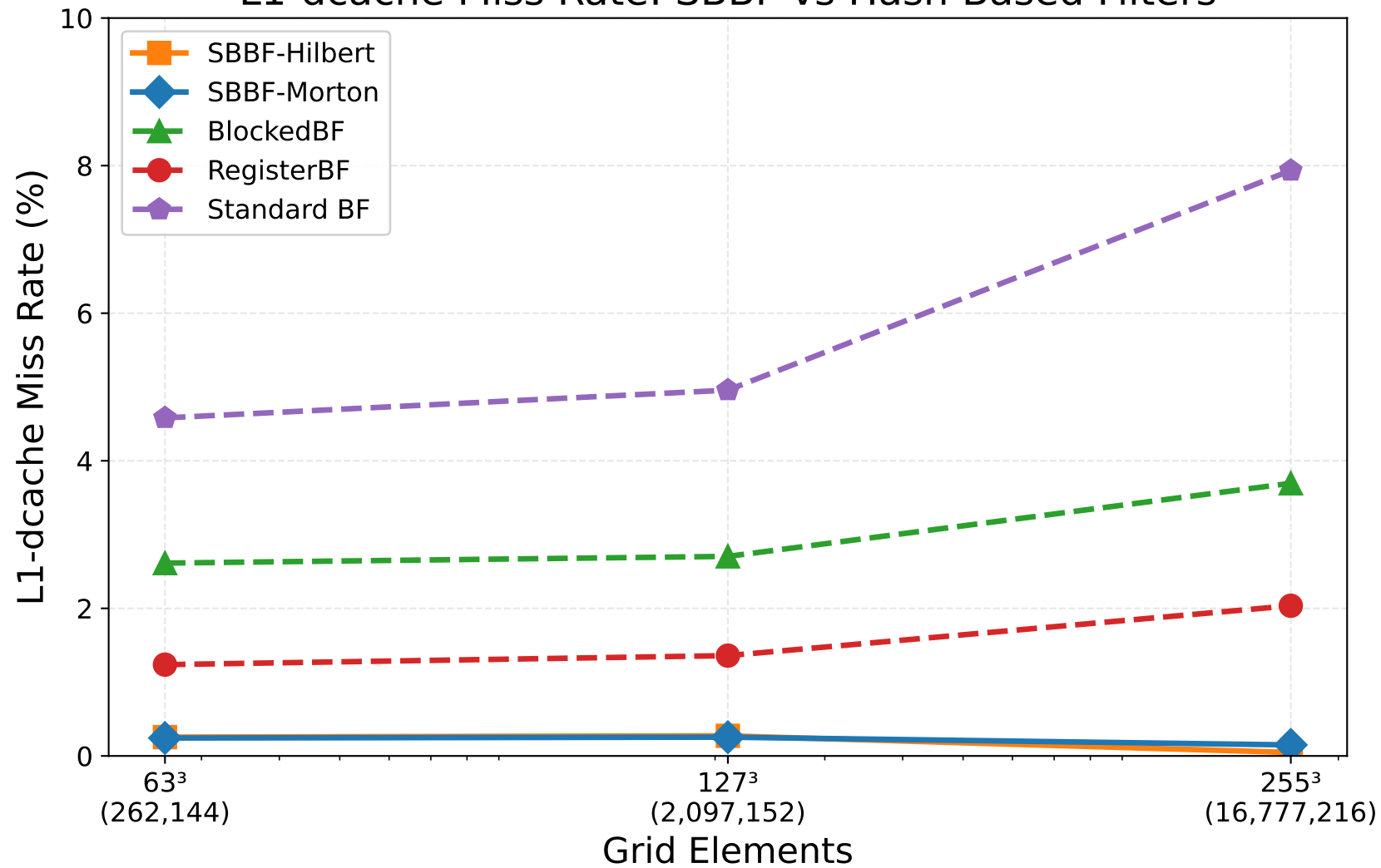
L1-dcache Miss Rate: SBBF vs Hash-Based Filters
