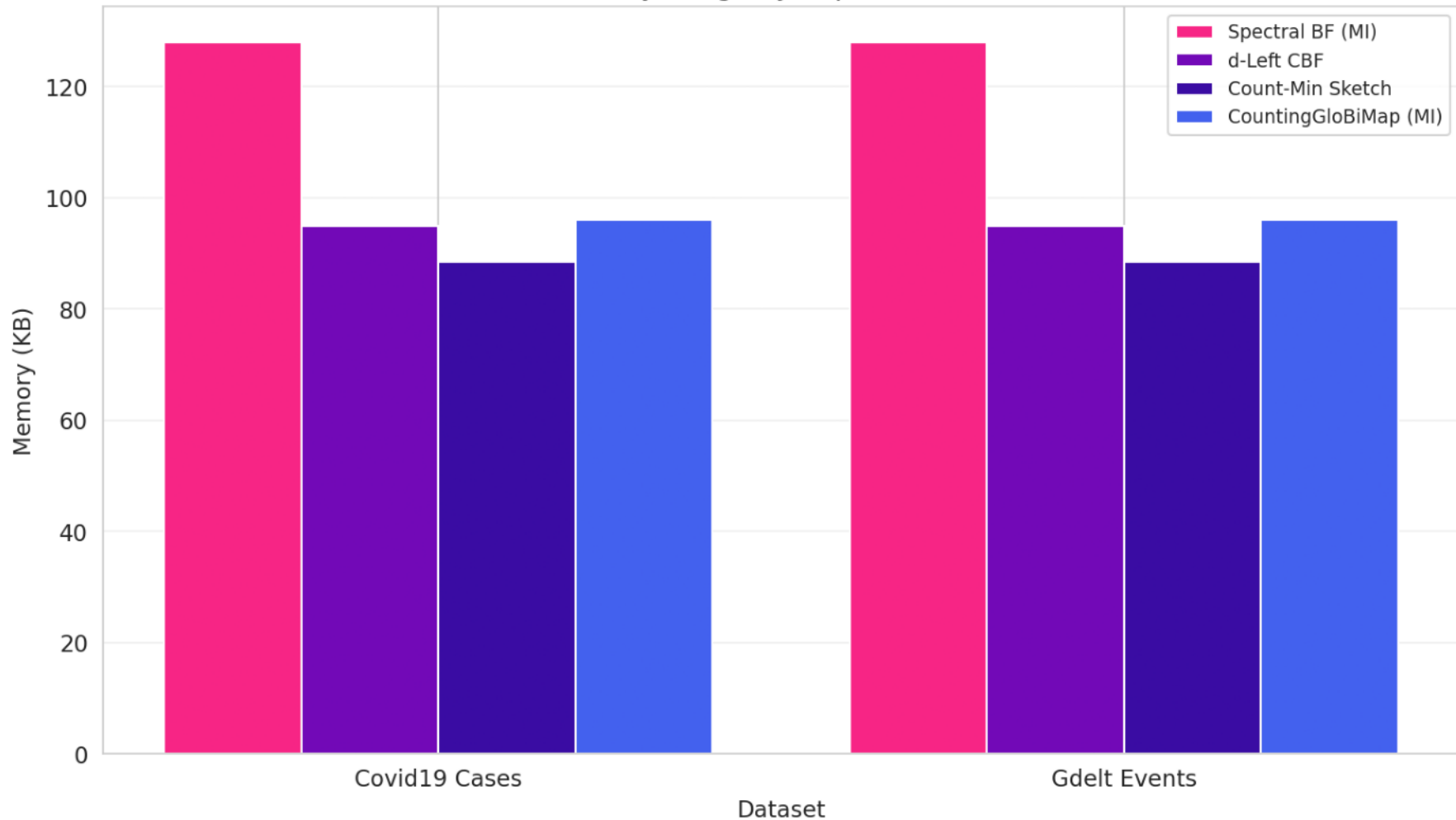
Memory Usage by Implementation
