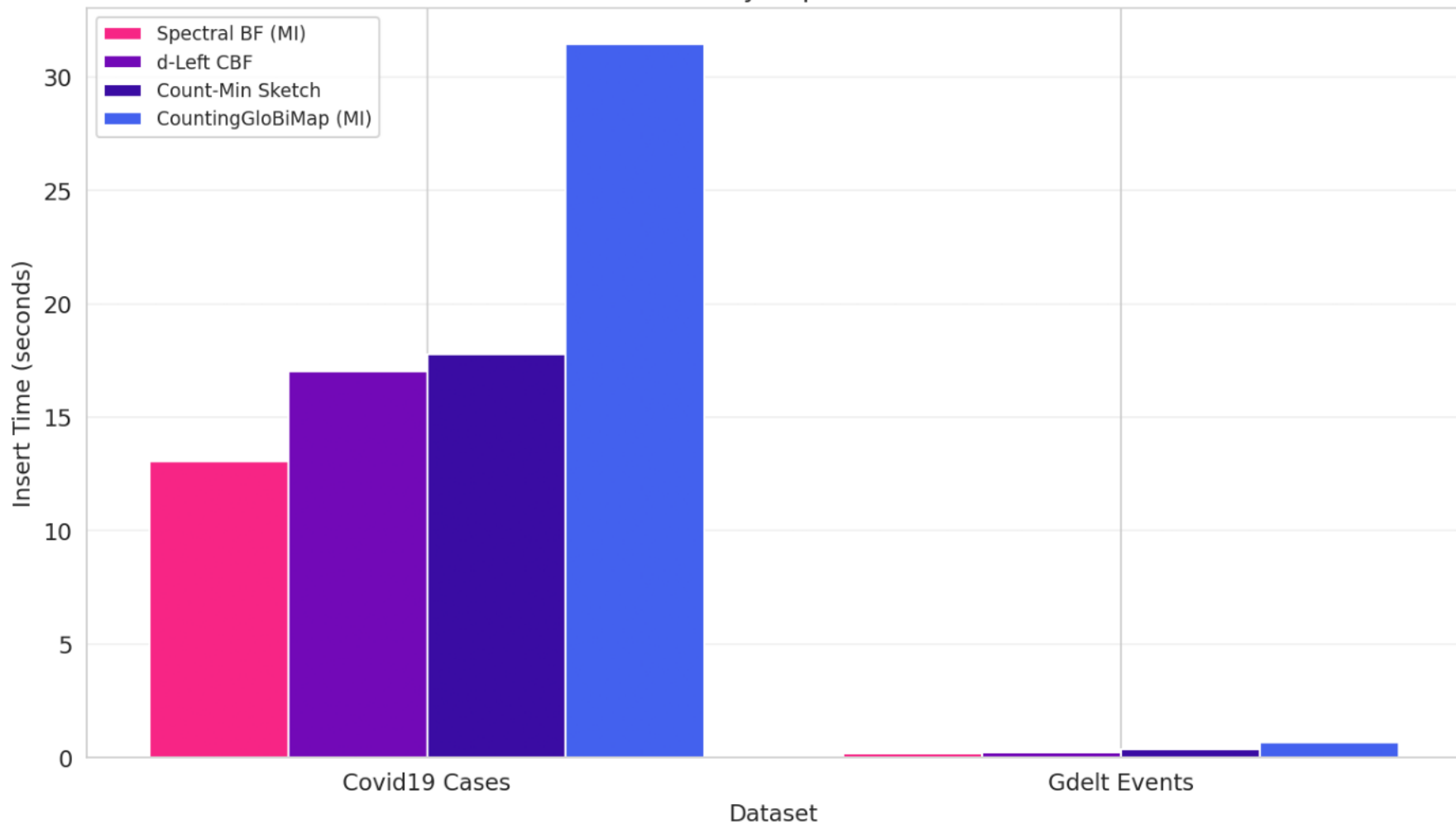
Insert Time by Implementation
