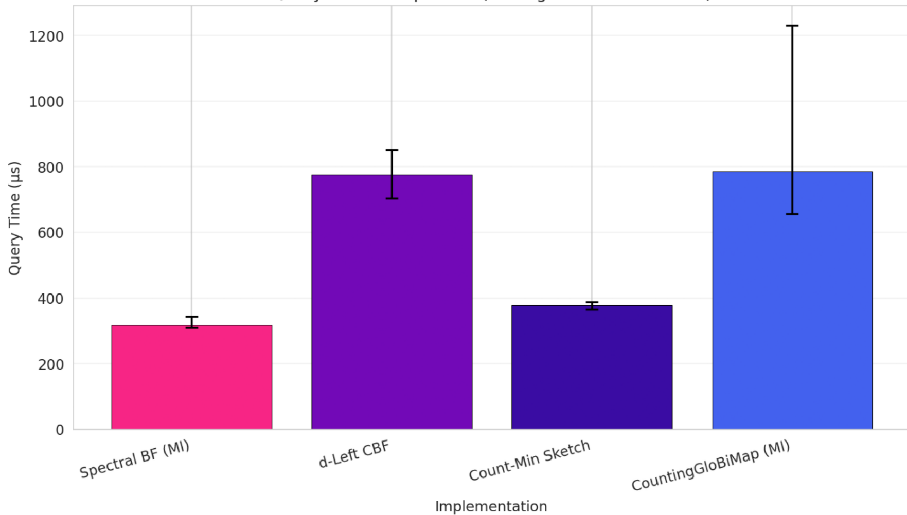
Query Time Comparison (averaged across datasets)
