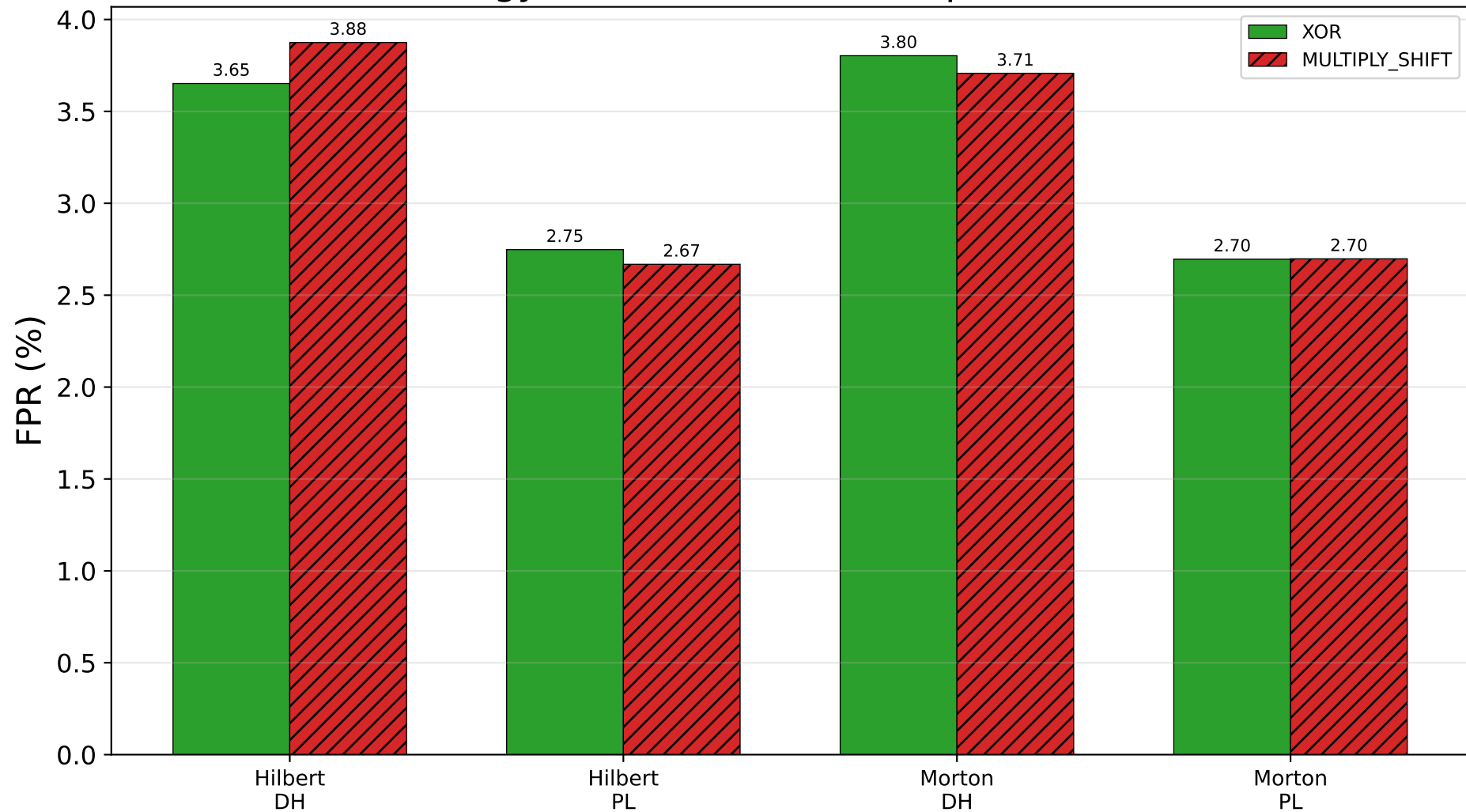
Seed Strategy: Clustered 2D (100K points, 50 clusters)
