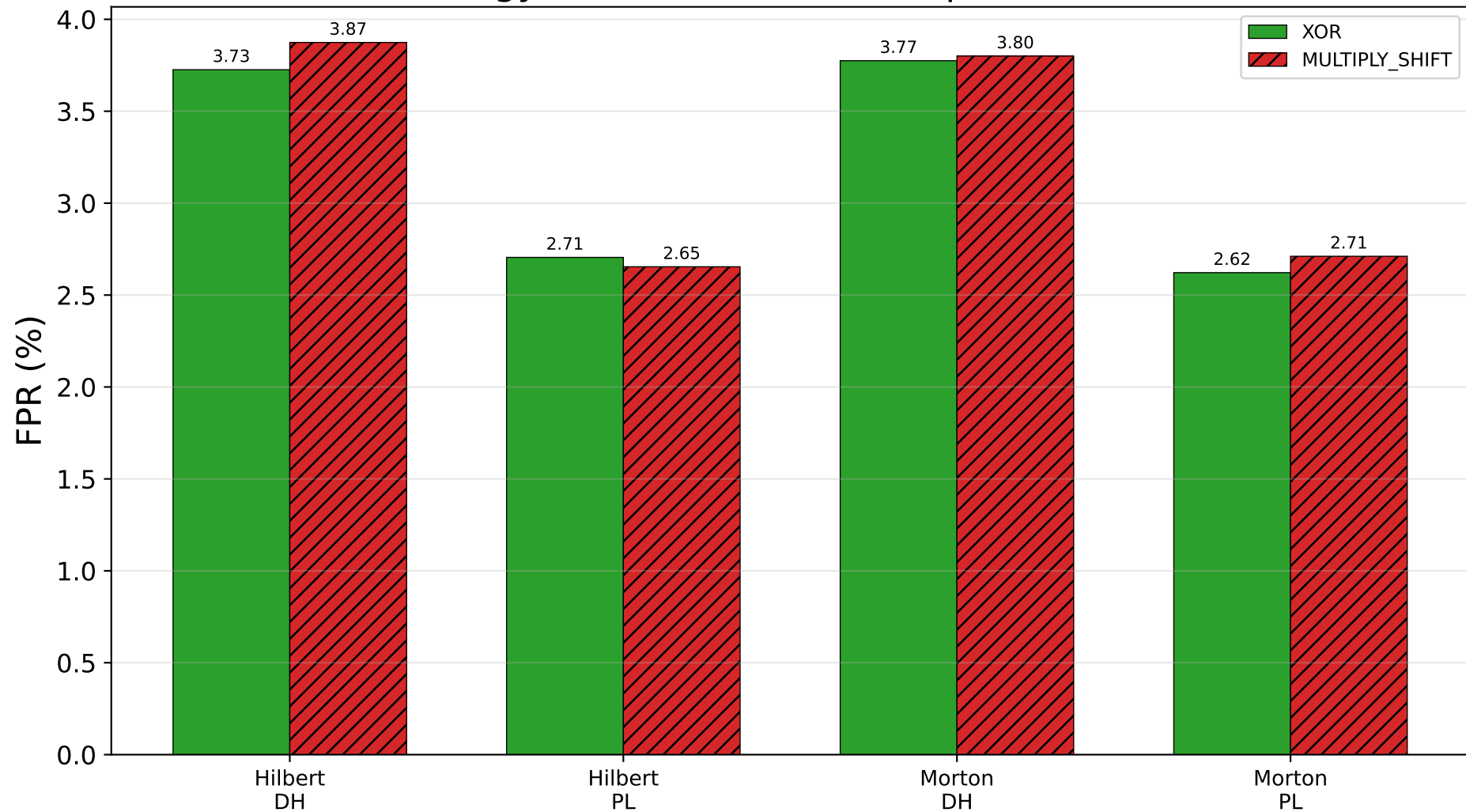
Seed Strategy: Clustered 3D (100K points, 50 clusters)
