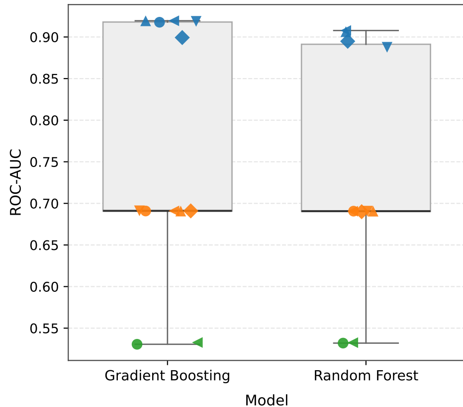
Figure 1. Overall model performance in terms of roc-auc and max aaod. Colors represent datasets, and marker shapes indicate the optimization metric.
