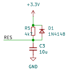
Power-up reset circuit
