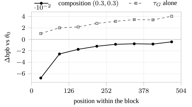
Figure 2: Per-token \Delta\text{bpb} against the backbone, by position within the 512-token block, in eighths. The composition’s gain is almost entirely spent in the first eighth, while the genre module on its own grows steadily more damaging as context accumulates. Negative is better than \theta_0 .
