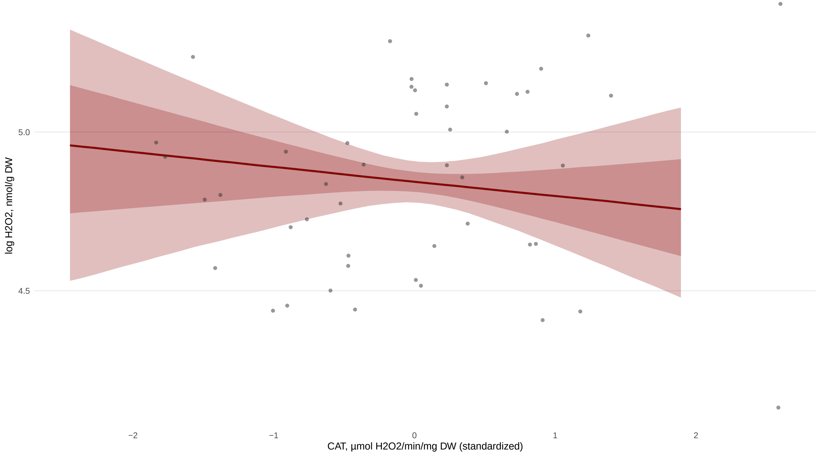
Posterior effect curve Posterior median with credible band(s), from model draws
