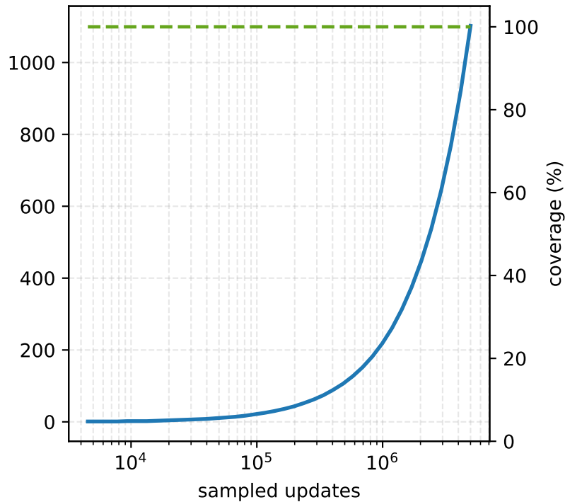
Systemic Risk
