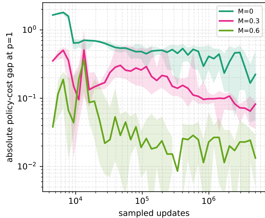
Systemic Risk
