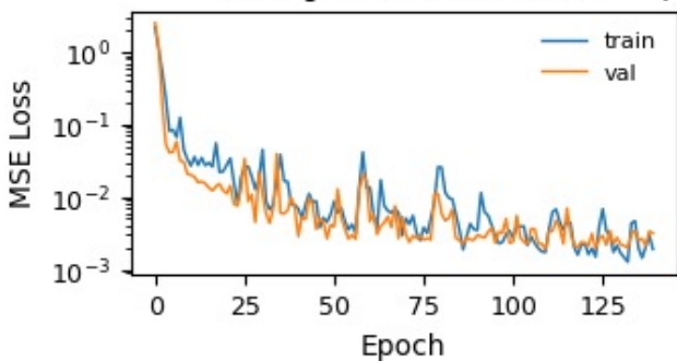
b Training and Validation Loss
