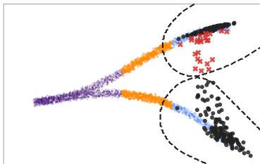
OT-CFM
