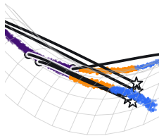
OT-CFM
