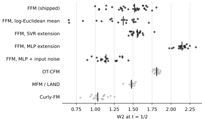
d = 2, pool
