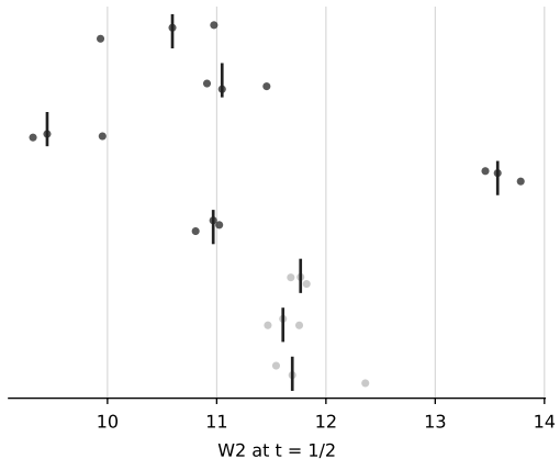
d = 10, seeds 0-2
