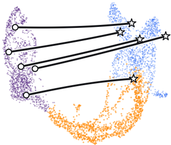
OT-CFM
