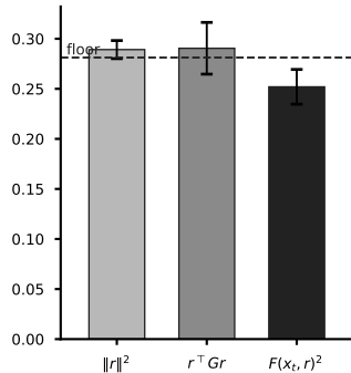
W_{2,F}
