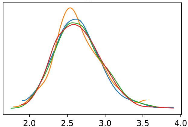
sigma_lambda
