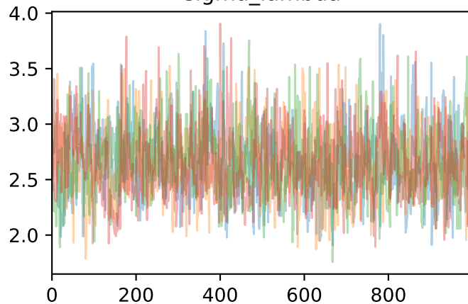
sigma_lambda
