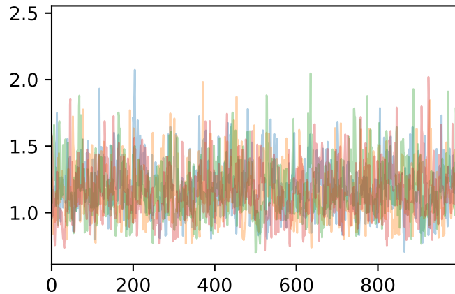
sigma_lambda
