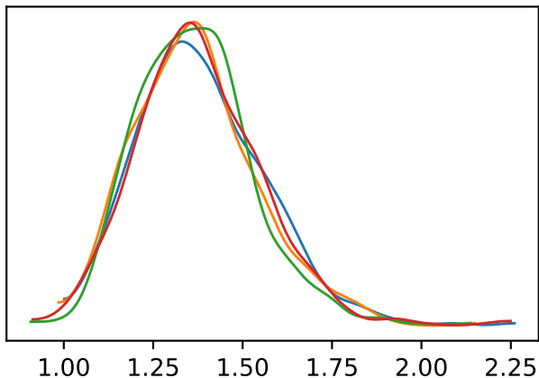
sigma_lambda
