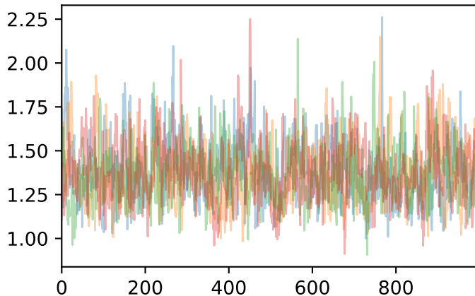
sigma_lambda
