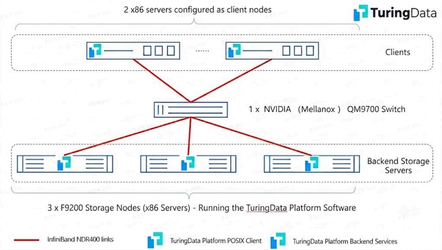
Hardware Diagram
