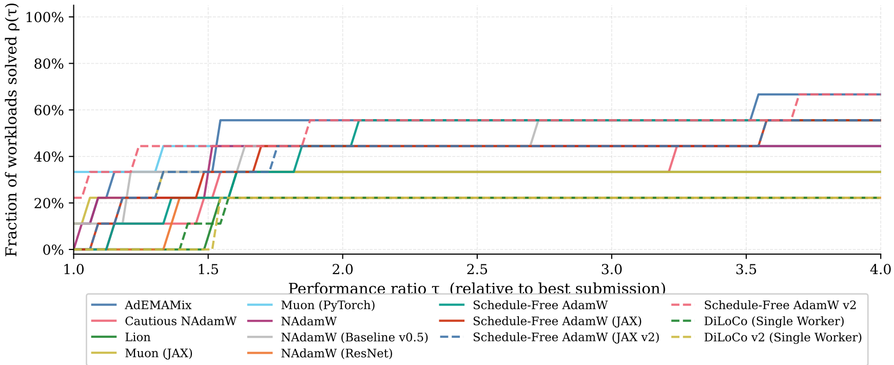
AlgoPerf: Self-Tuning Performance Profiles (steps to target)
