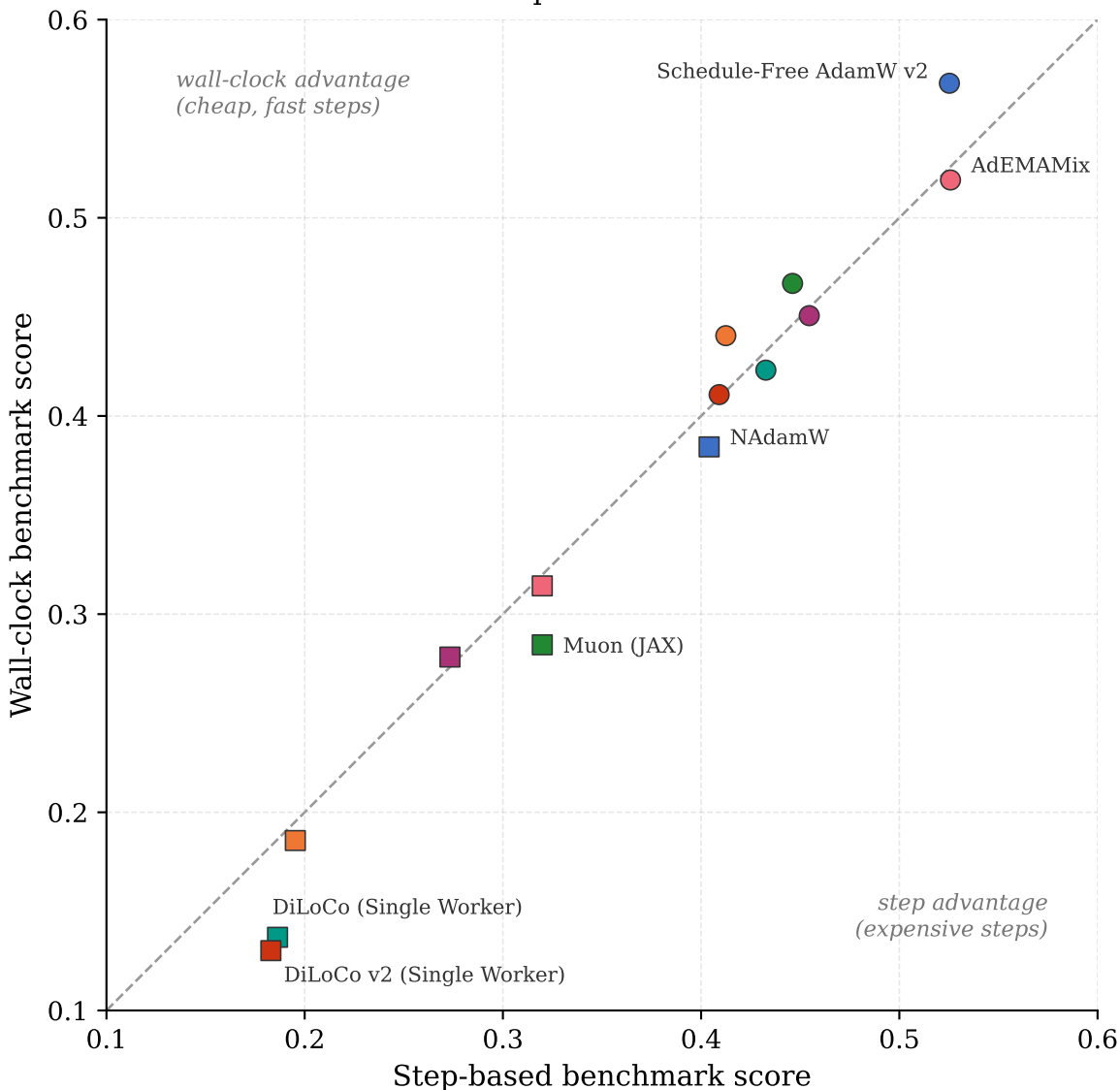
Wall-clock vs. step-based benchmark scores
