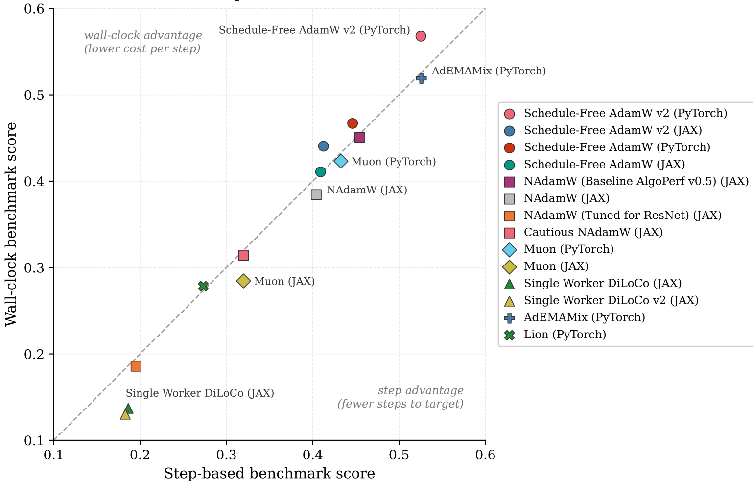
Wall-clock vs. step-based benchmark scores
