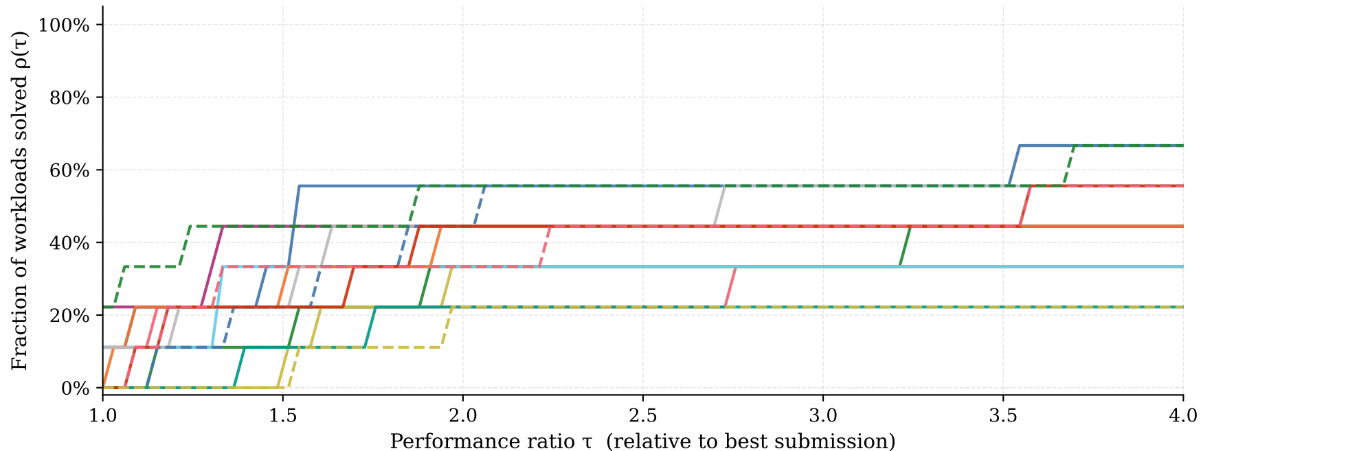
AlgoPerf: Self-Tuning Performance Profiles (steps to target)
